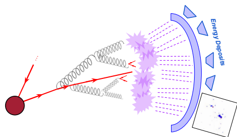
Observed Jet
